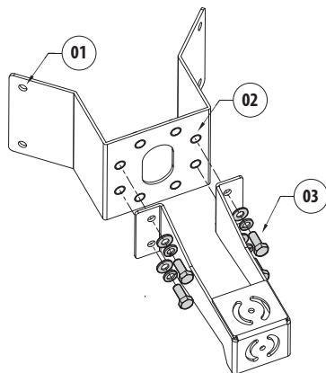
Fig. 2 Fastening for Esprit Anti-Corrosion Fixed (Pelco), NTX (VIDEOTEC).
