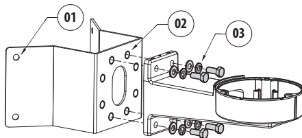
Fig. 1 Fastening for UEBW (Esprit Compact (Pelco), ULISSE EVO DUAL (VIDEOTEC)).
